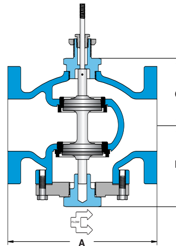
Stem In-to-Open (normally closed)
